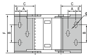
X 3 type bracket
